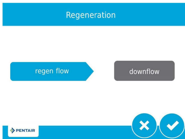
Figure 22 Regeneration Screen
